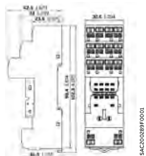
CR-MxLP - push-in connection
