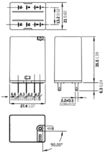
CR-M relay with 2 c/o contacts
