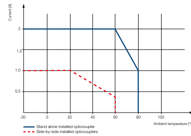
Derating curve Triac output CR-S
