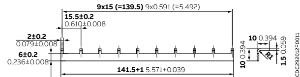
CR-PJ jumper bar
