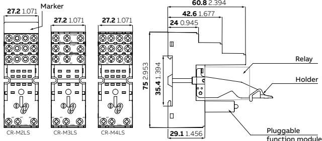
CR-M2LS(H) - CR-M3LS(H) - CR-M4LS - screw connection
