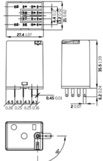
CR-M relay with 4 c/o contacts
