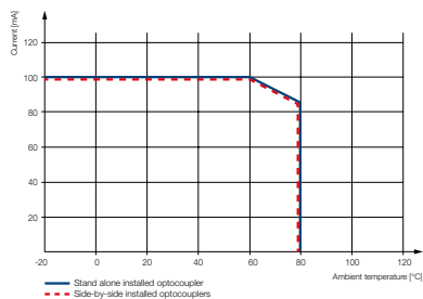
Derating curve Transistor output CR-S
