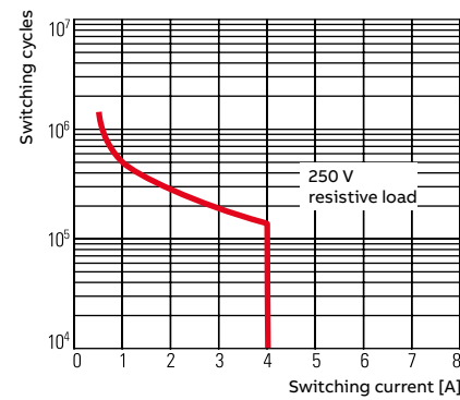
Contact lifetime
