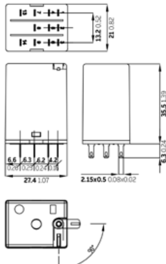
CR-M relay with 3 c/o contacts
