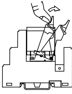
Removal
