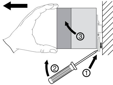
Dismounting
